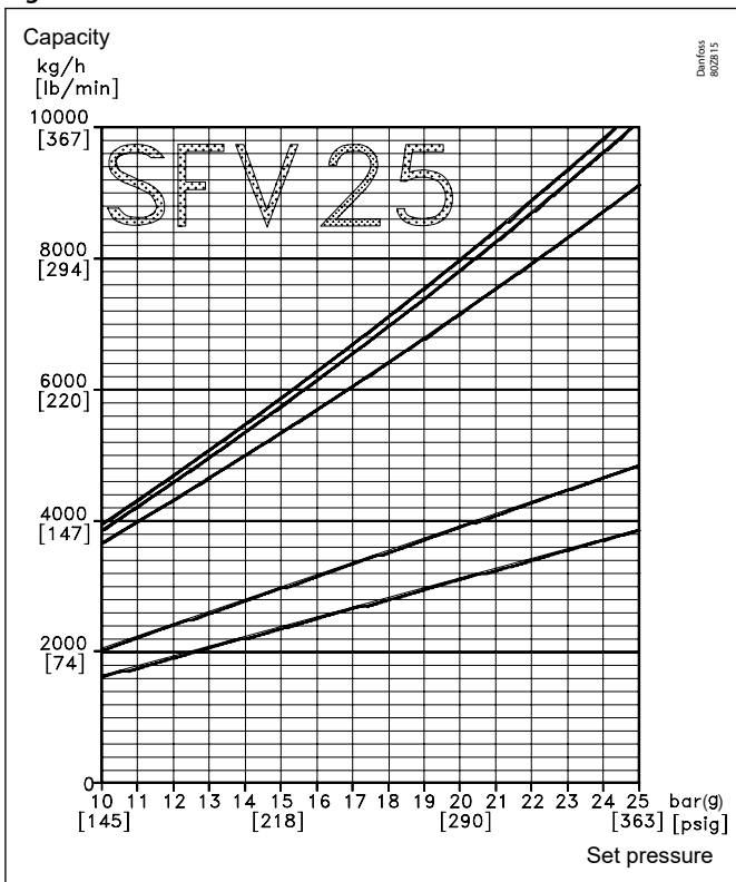
Figure 5: SFV 25
