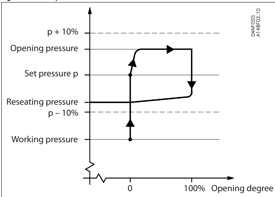
Figure 1: SFV Graph
